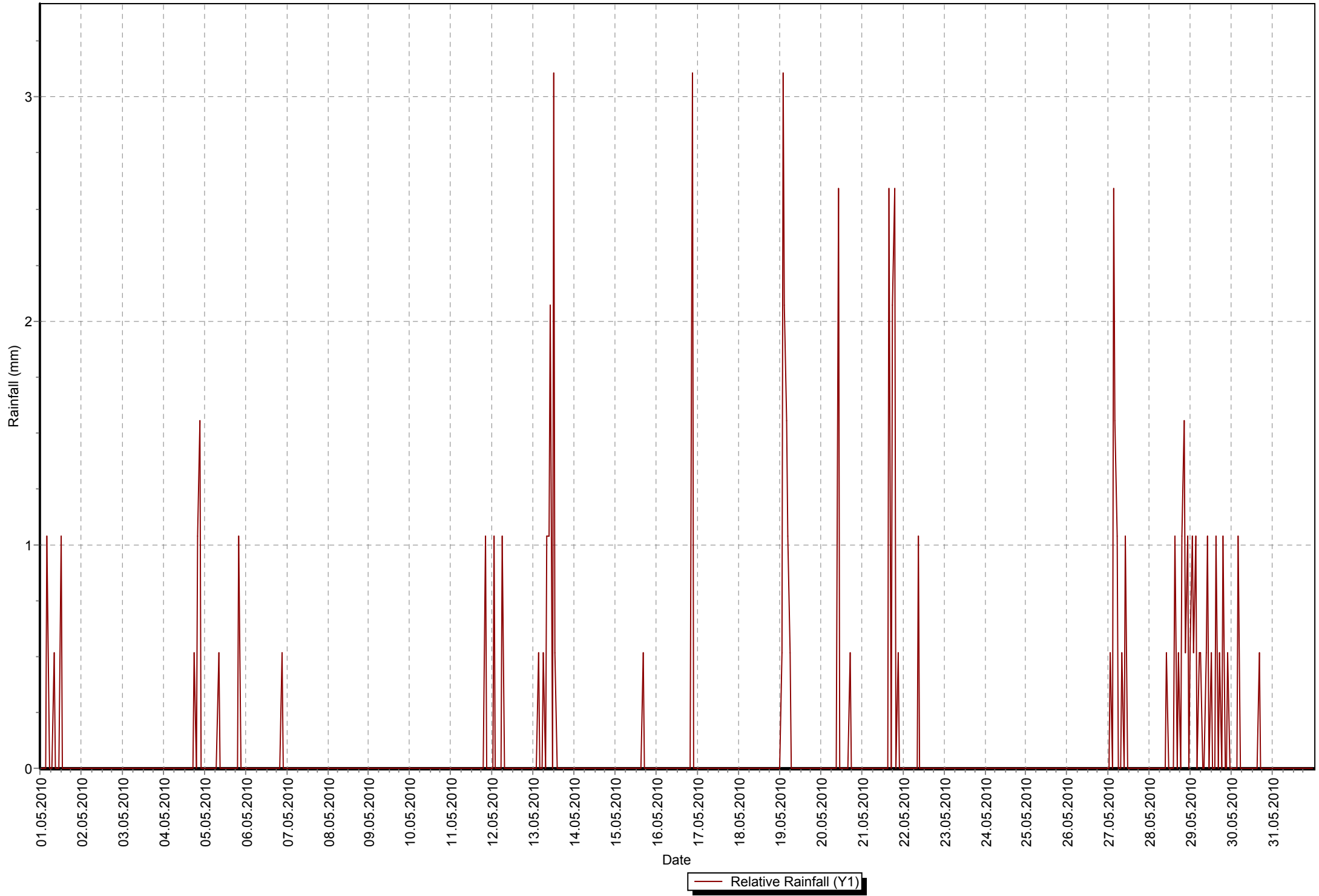
Milovaig Rainfall - May 2010
