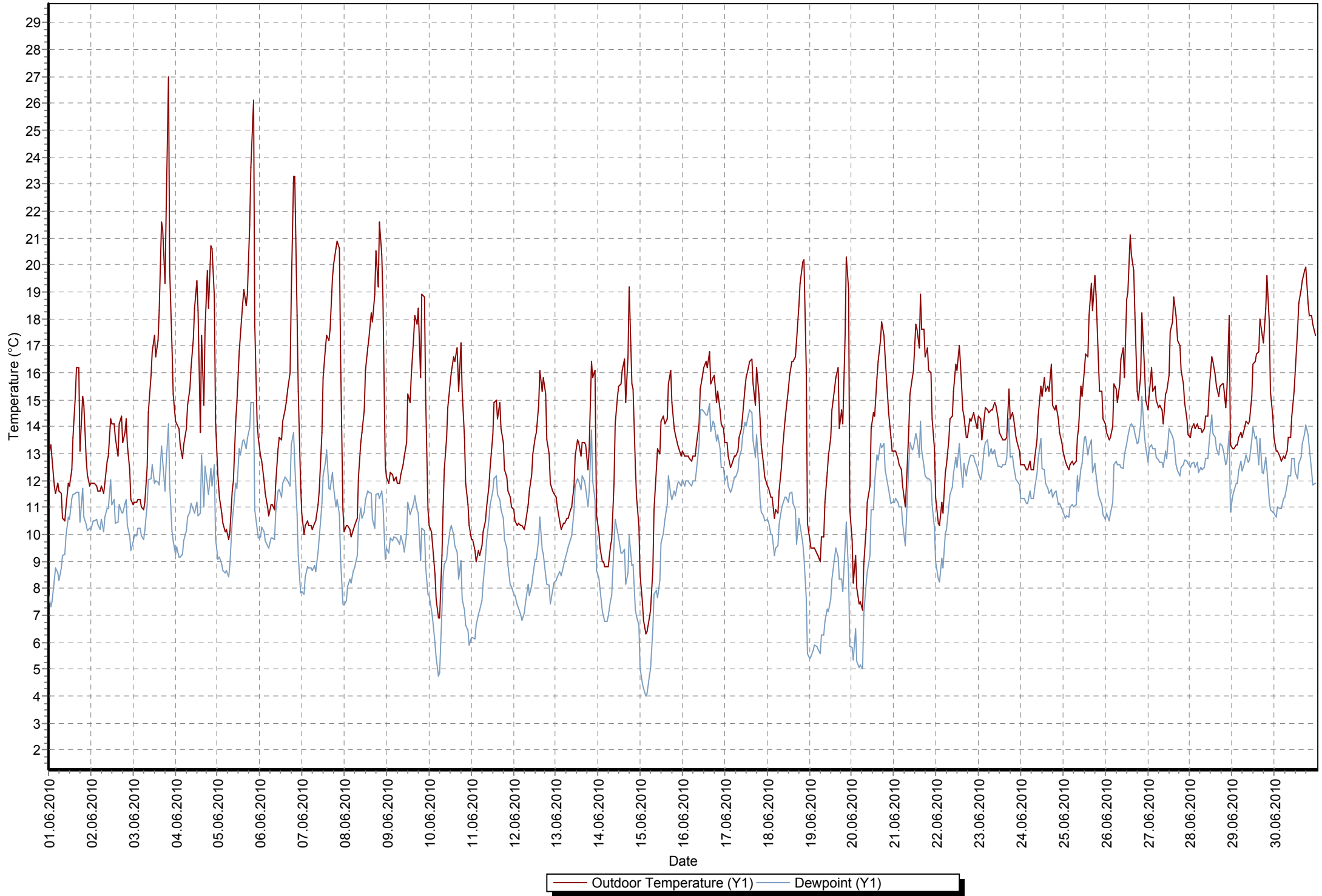
Milovaig Dewpoint - June 2010
