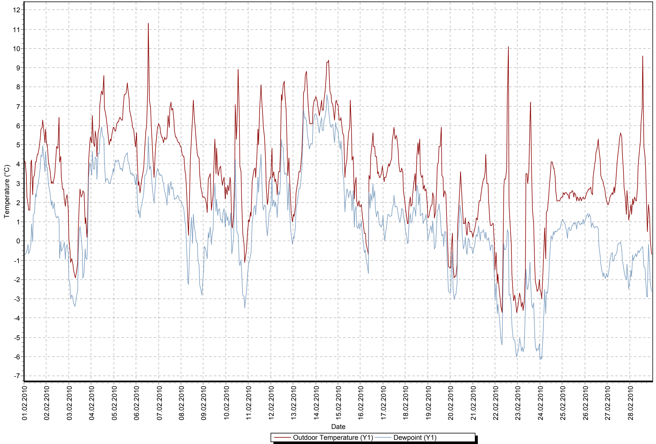
Milovaig Dewpoint - Feb 2010
